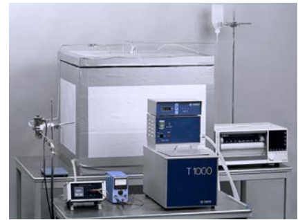
Fluid susceptibility cabinet
