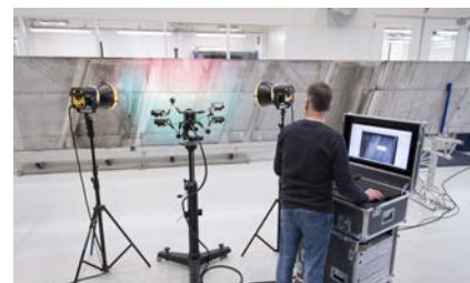
Shearography on wing flap
